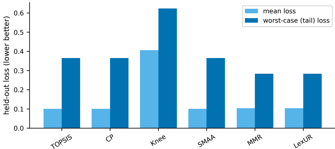
Smart-grid: held-out decision loss by method
