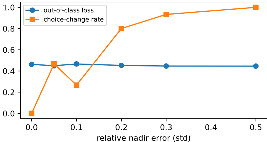
LUR sensitivity to nadir error (concave, m=8 )
