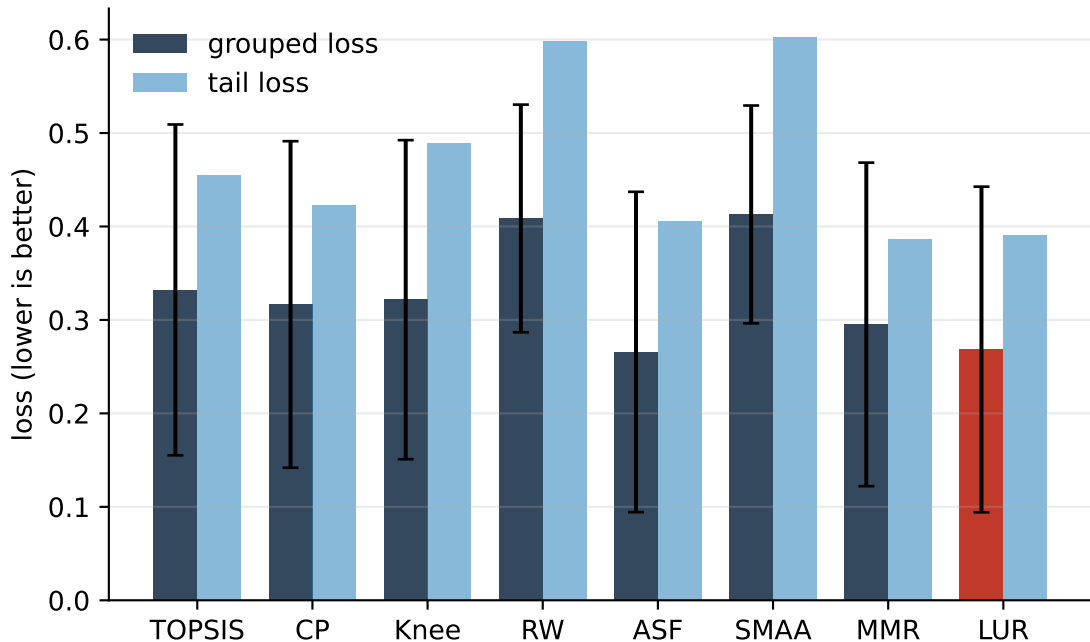
Robustness to redundant criteria (grouped vs tail loss)
