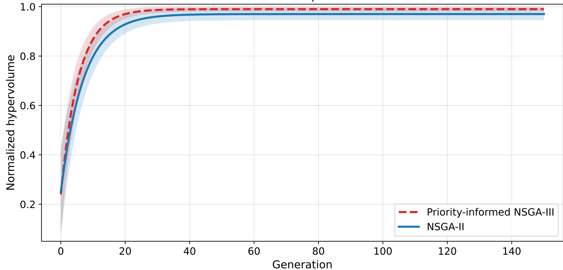
Hypervolume convergence on the 10-profile plan mean \pm 1 std across profiles and seeds
