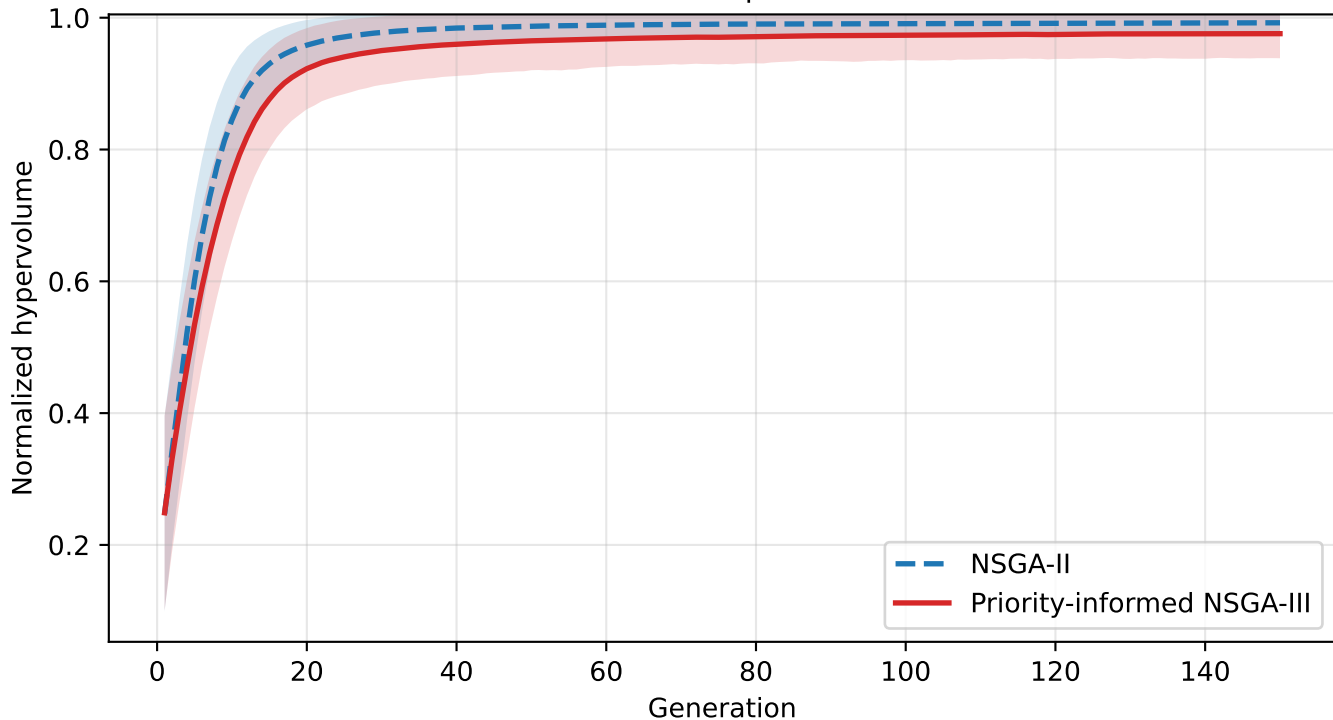
Hypervolume convergence on the 10-profile plan mean \pm 1 std across profiles and seeds
