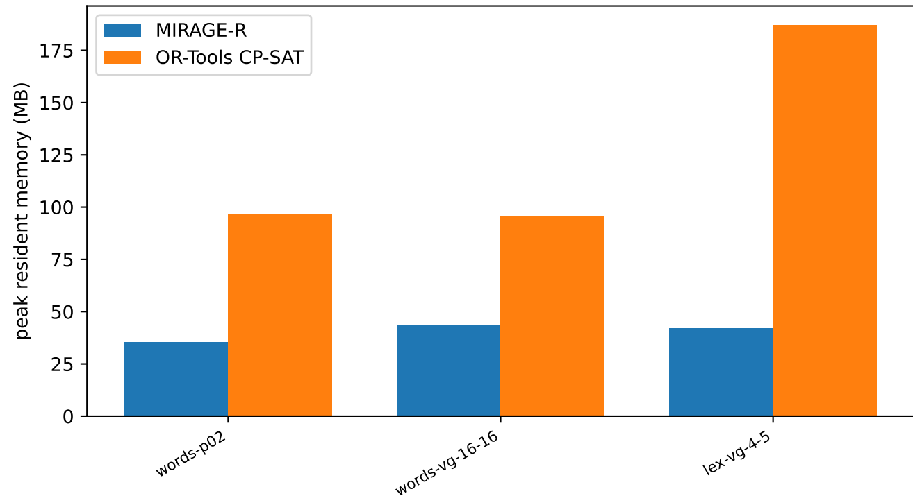
Peak memory footprint: MIRAGE-R vs CP-SAT
