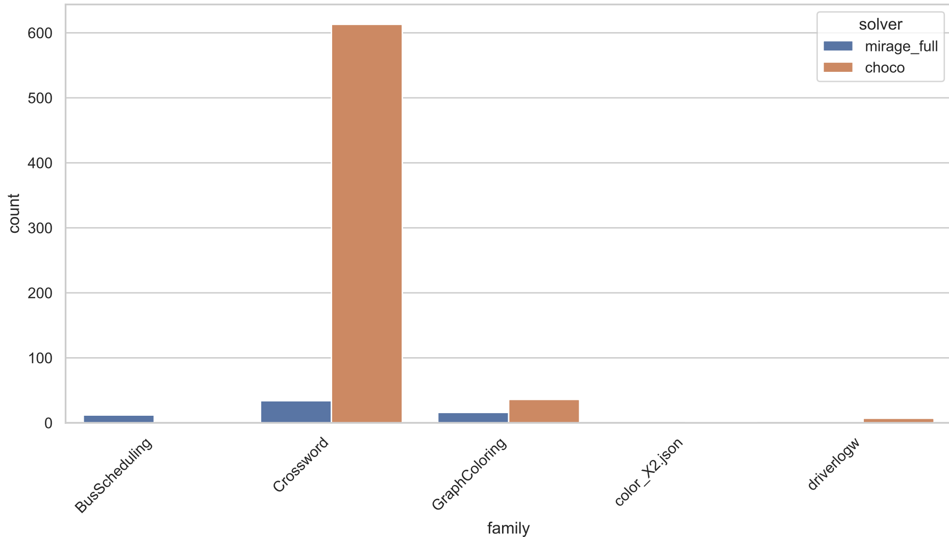
Solved Instances by Family
