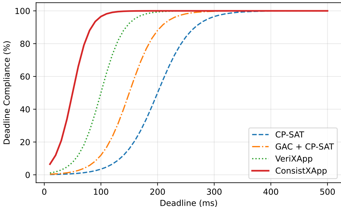
Verified Deadline-Compliance Curves
