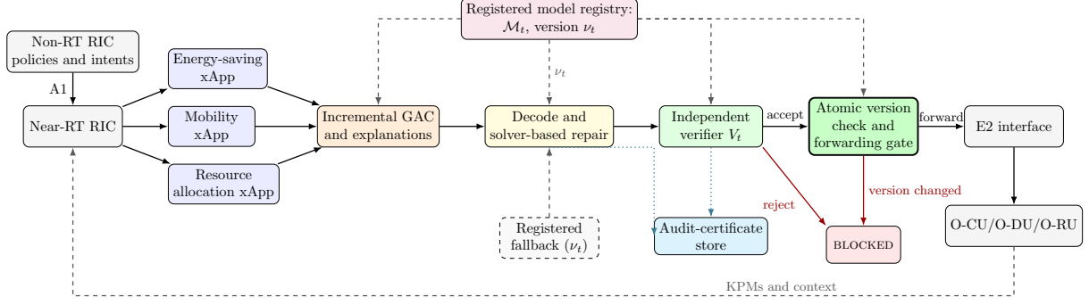
Fig. 1 CONSISTXAPP in the Near-RT RIC control path. Solid arrows carry control proposals and accepted actions; dashed arrows carry registered-model and context data; dotted arrows carry audit data. Every forwarded action passes the independent verifier V_t and an atomic model-version check bound to \nu_t : a candidate rejected by the verifier, or one whose model version changed between verification and forwarding, is not admitted to E2. Incremental GAC and solver-based repair generate candidates efficiently but are outside the trusted path—a fault in either can reduce availability or objective quality, but cannot by itself cause a registered-model-invalid forwarding.
