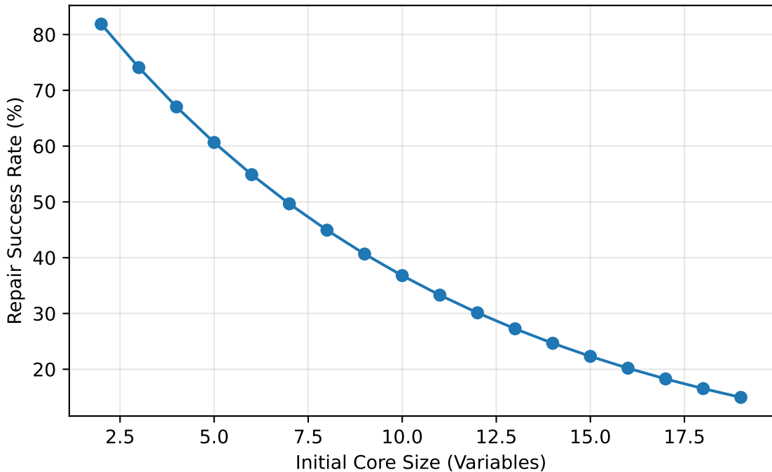
Repair Success Rate vs. Initial Core Size
