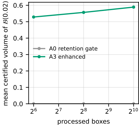
A. Anytime progression
