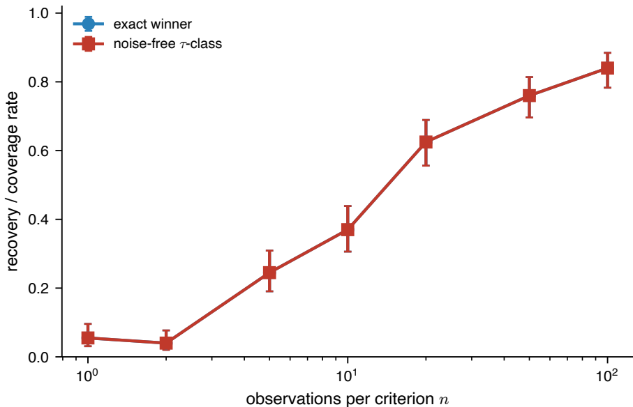
Confidence-aware LexPR recovery (concave, m = 6 )
