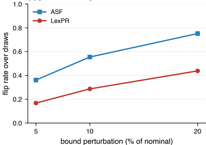
(c) point-winner flip rate
