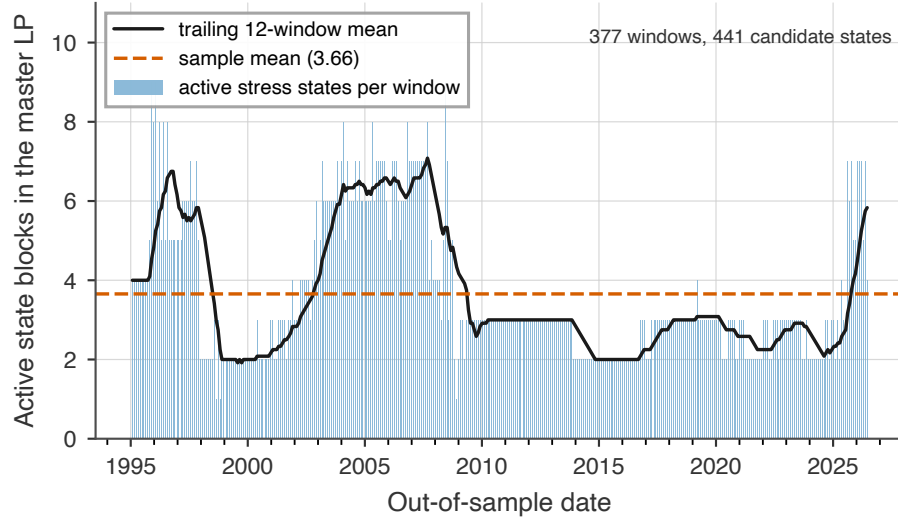
Fig. 10 Active state blocks across rolling windows
