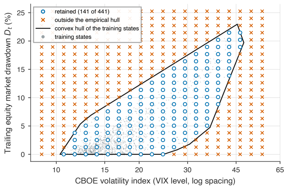
Fig. 16 Candidate states retained after restriction to the empirical convex hull of the training sample, for a representative rolling window. Circles mark retained states, crosses mark those excluded, and the solid line is the hull boundary
