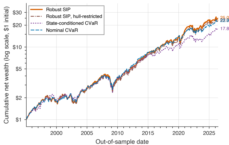
Fig. 17 Cumulative out-of-sample wealth of the support-restricted and state-conditioned specifications against the baseline and the strongest unconditional benchmark, net of 10 basis points per unit of turnover
