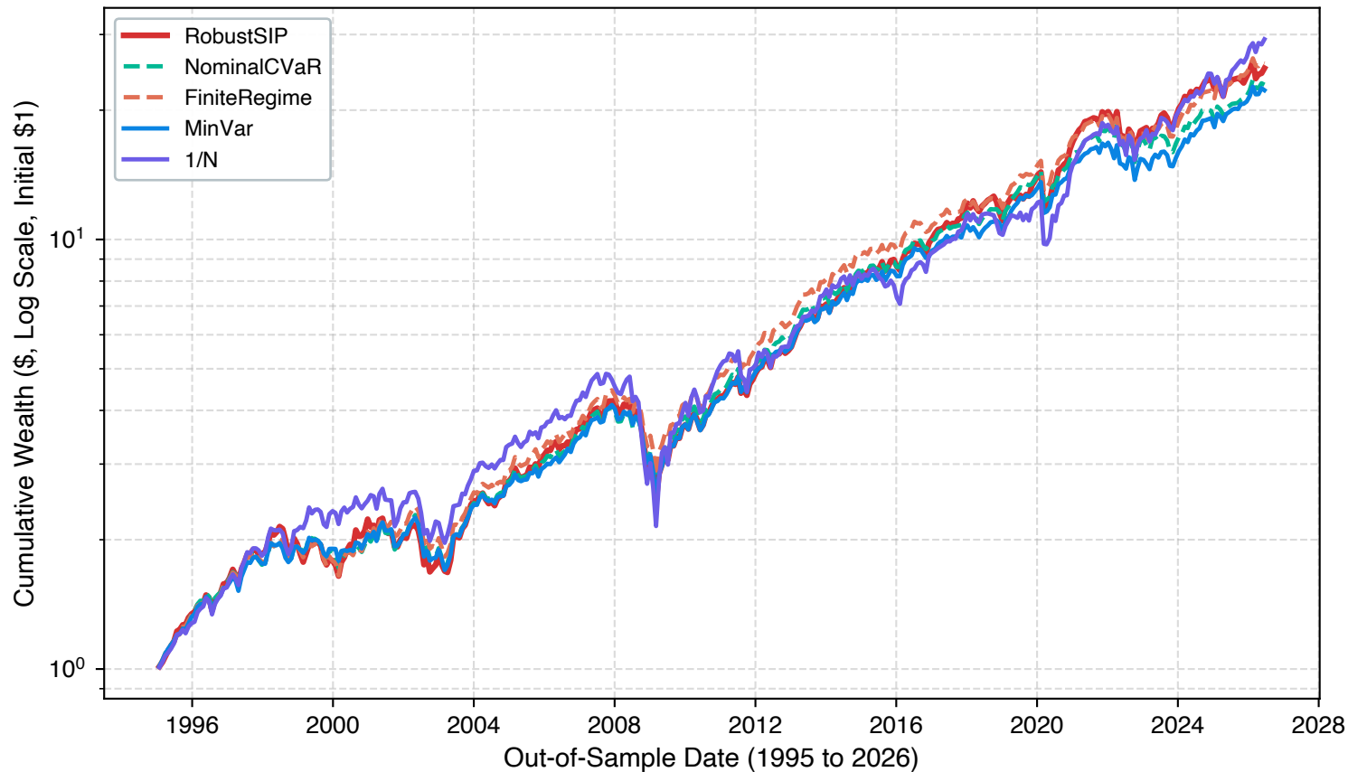
Out-of-Sample Cumulative Net Wealth Trajectories (Net of 10 bps TC)
