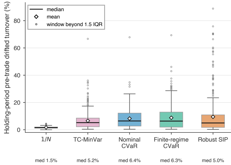
Fig. 8 Distribution of holding-period portfolio turnover.
