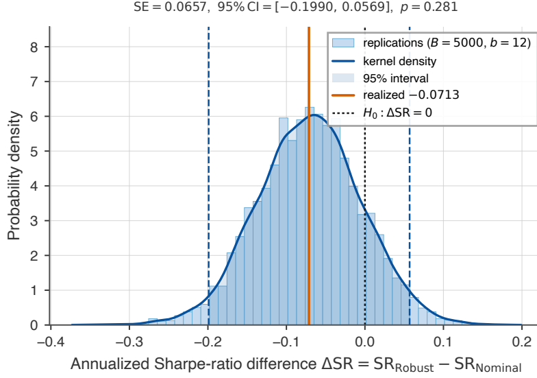
Fig. 15 Bootstrap distribution of the Sharpe-ratio difference.
