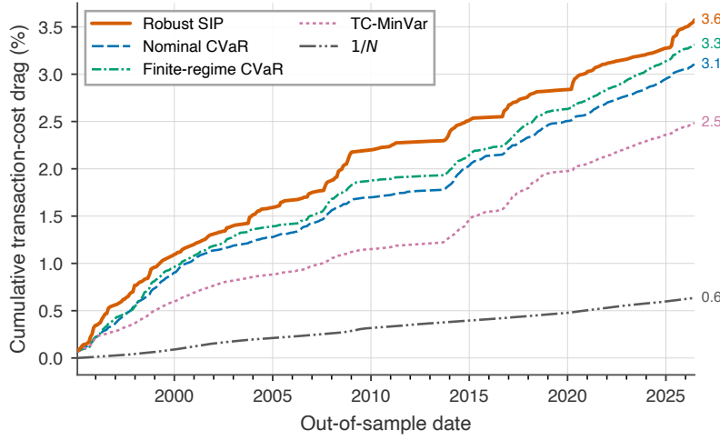
Fig. 9 Cumulative transaction cost impact.
