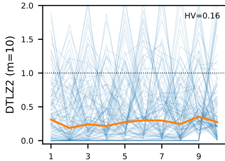
HLLDBEA strict
