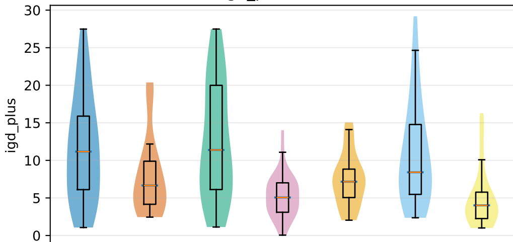
Final igd_plus distribution
