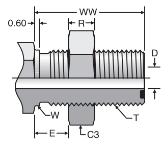
Seal-Lok Bulkhead
