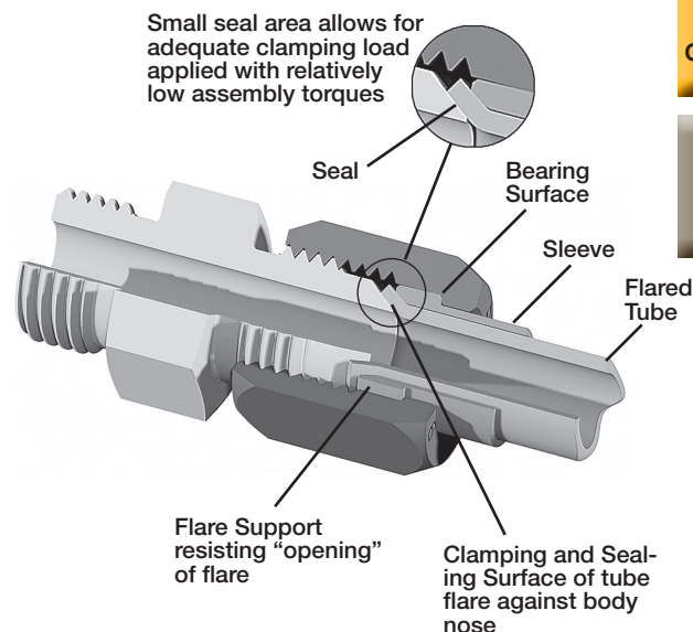
Fig. B1 – Triple-Lok Design and Features
