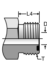
Seal-Lok Male Tube End
