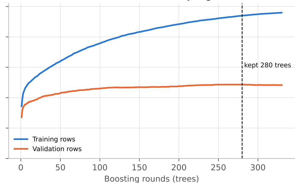
XGBoost, no resampling
