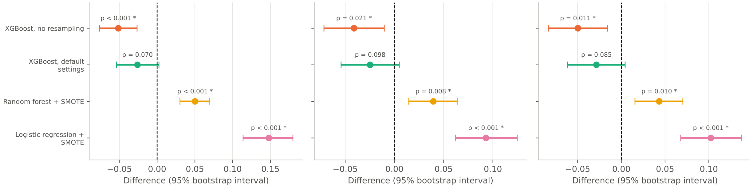
PR-AUC: proposed minus other
