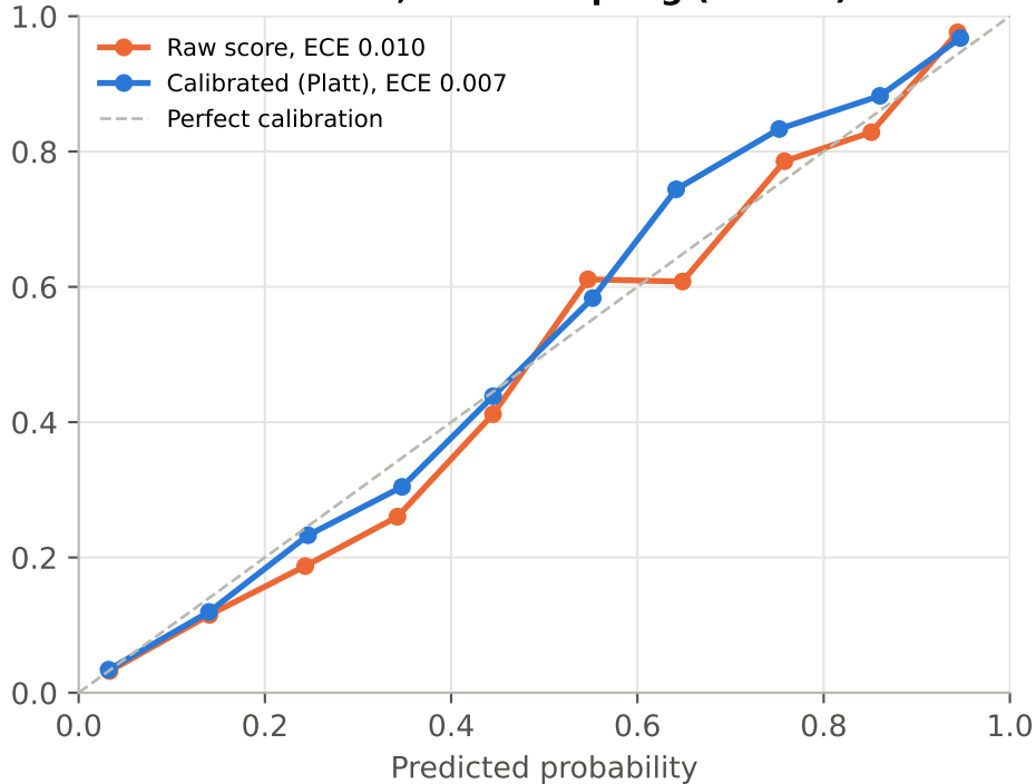
XGBoost, no resampling (served)
