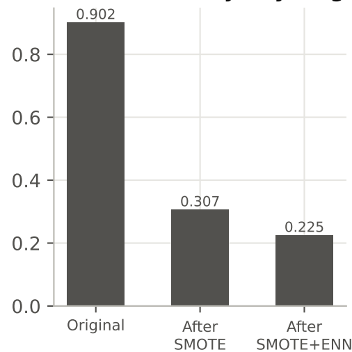
Boundary noise, theft rows (share with honest-majority neighbours)
