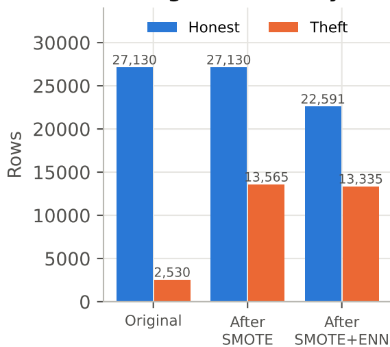
Training customers by class
