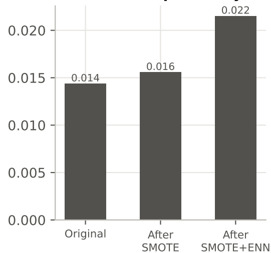
Mean Fisher ratio (feature separability)
