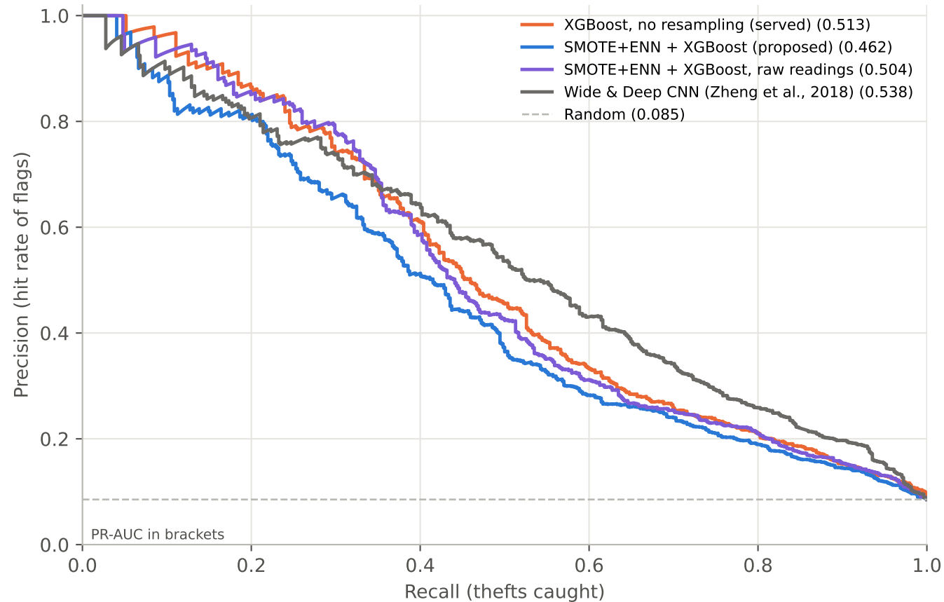
Precision-recall on the test customers, with the added pipelines
