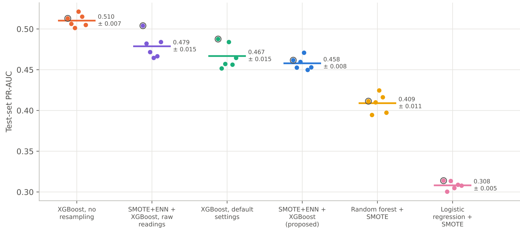
PR-AUC on 6 different random splits (circled: the study's split)
