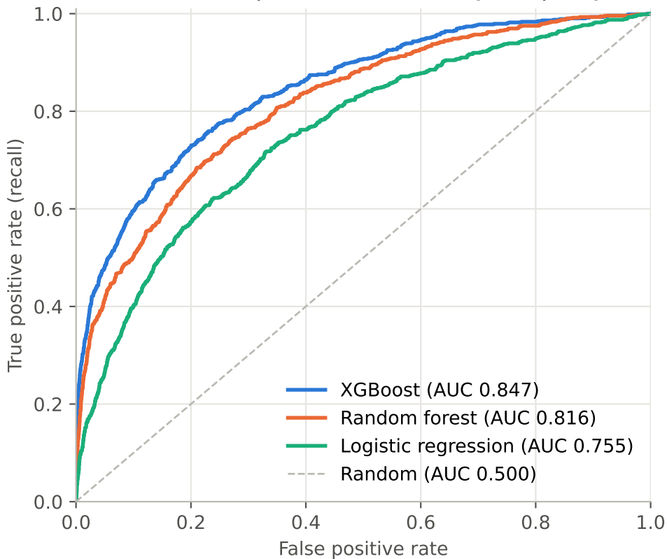
ROC curves, hold-out test set (n = 8,475)
