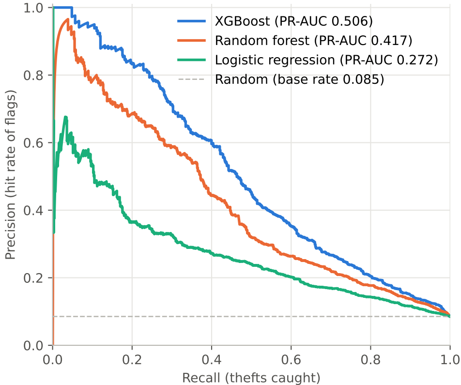
Precision-recall curves, hold-out test set
