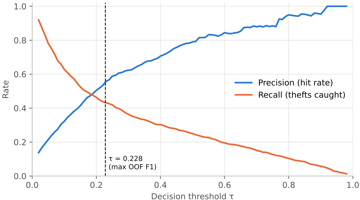
Precision and recall across thresholds, hold-out test set
