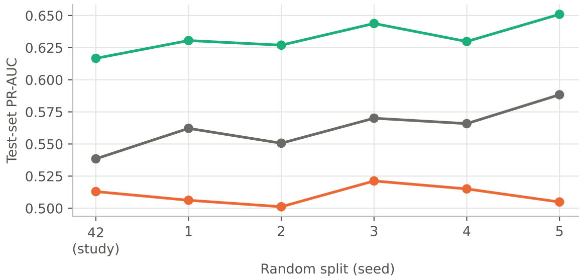
Hybrid ensemble against its two parts on six random splits (CNN weight 0.55 on every split)
