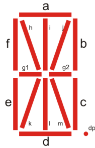
Figure 2.2: 14-Segment LED Alphanumeric Display
