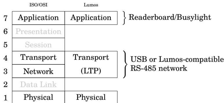
Figure 2.1: Protocol Stacks (ISO vs. Lumos Models)
