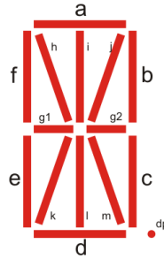
Figure 2.2: 14-Segment LED Alphanumeric Display
