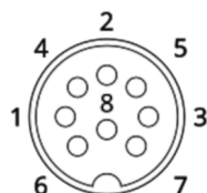
Figure 4.2: DIN-8 Jack (looking into socket from front)
