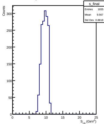
S_{\gamma N} apres coupures
