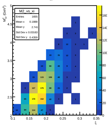
M_{\gamma p}^2 vs \xi
