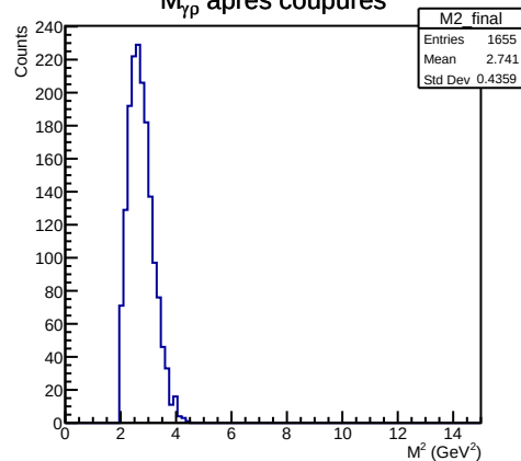
M_{\gamma p}^2 apres coupures
