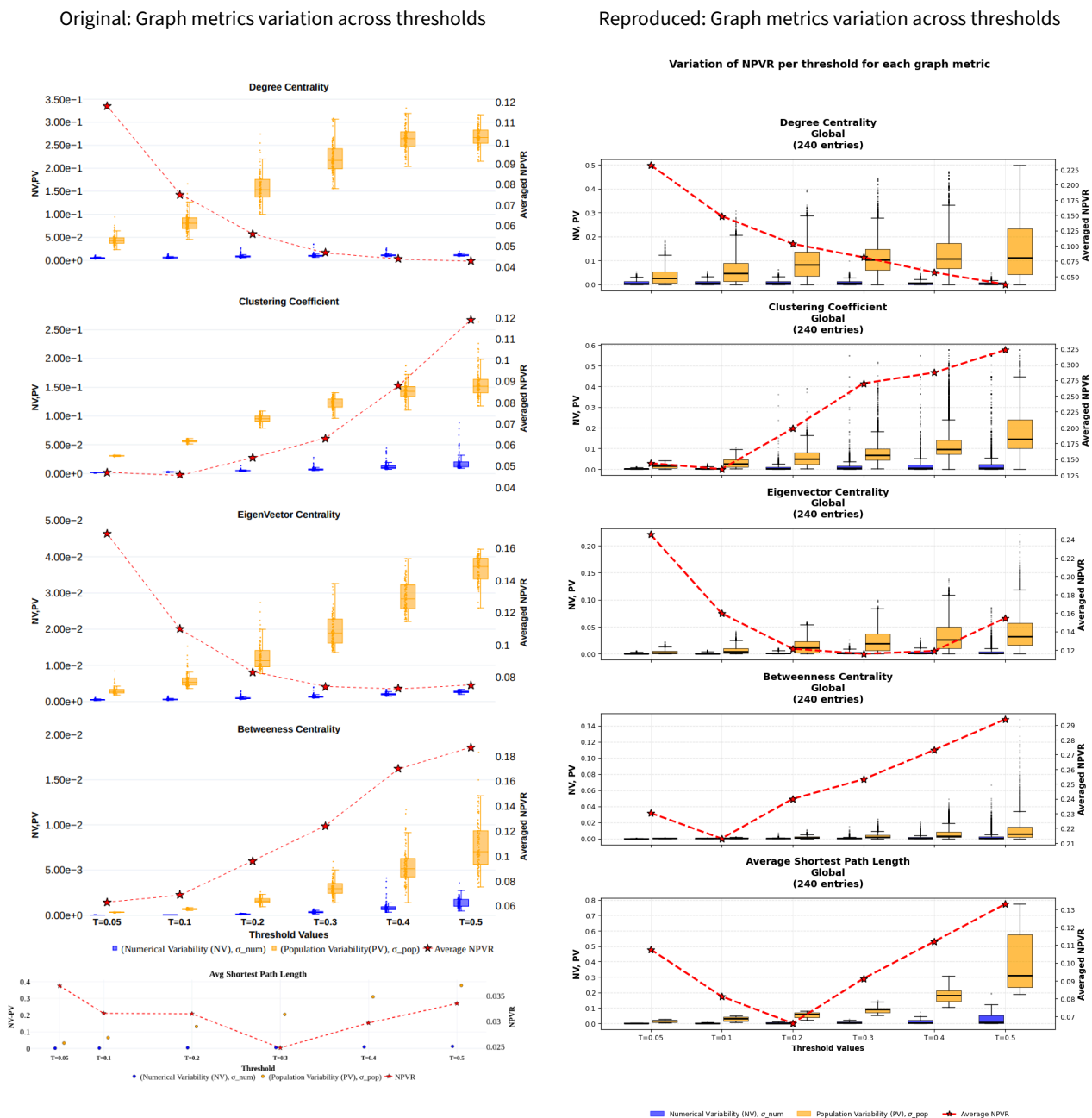
Figure 7 - Comparison of the original and reproduced NPVR values across graph metrics and thresholds
