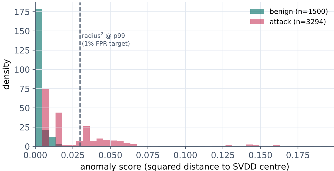
Deep-SVDD anomaly score — benign packs near the centre, attacks spread out
