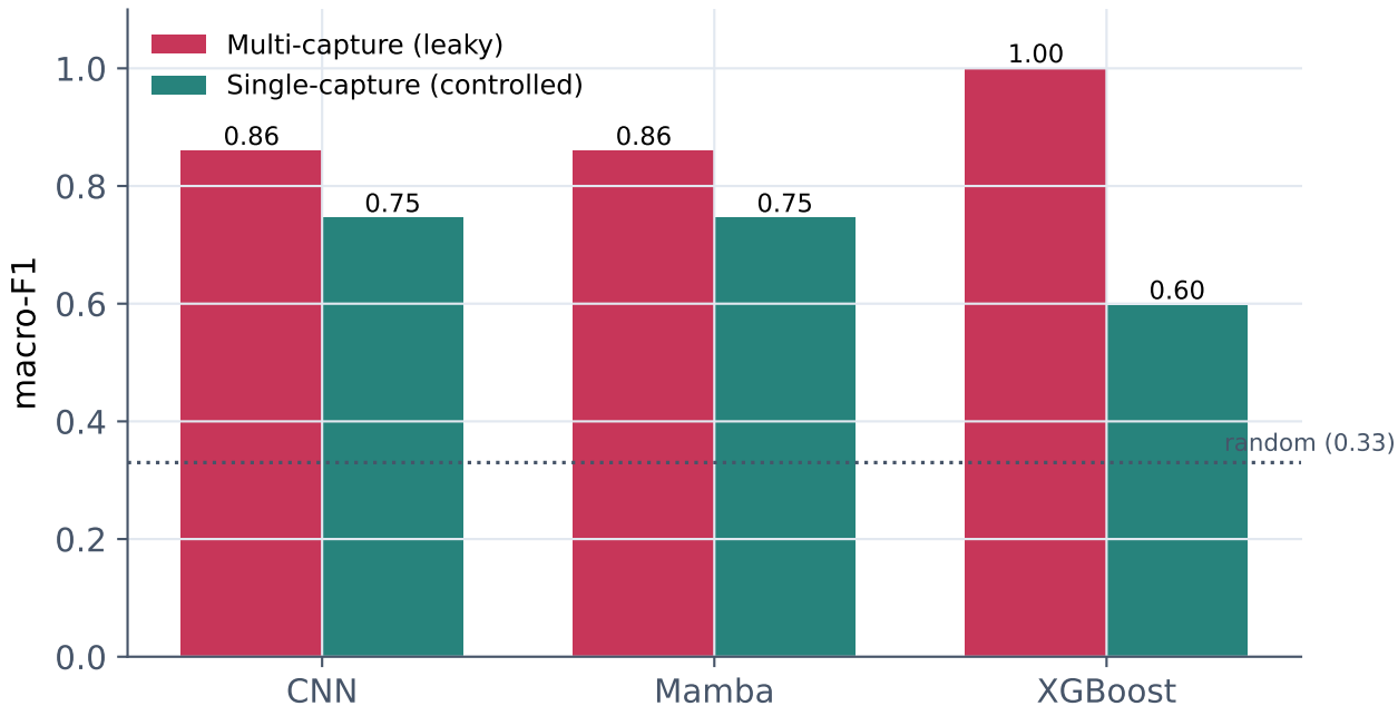
Sub-classifying Recon/DDoS/Mirai — capture leakage inflates naive numbers
