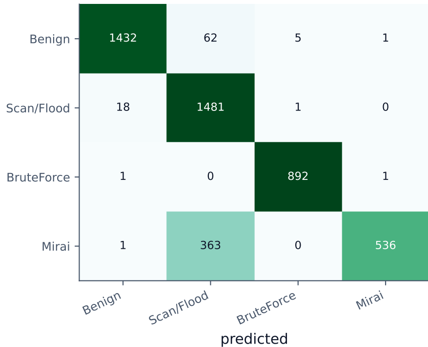
4-class (acc 0.906)
