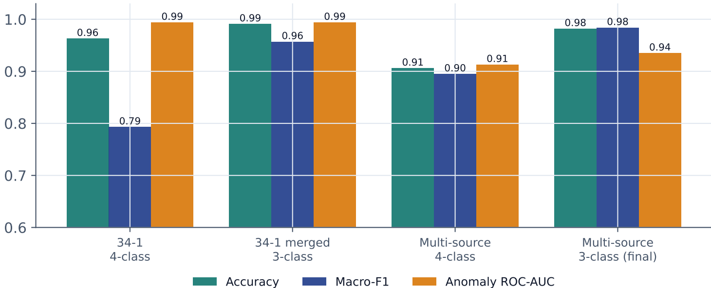
Metric evolution across the experimental journey
