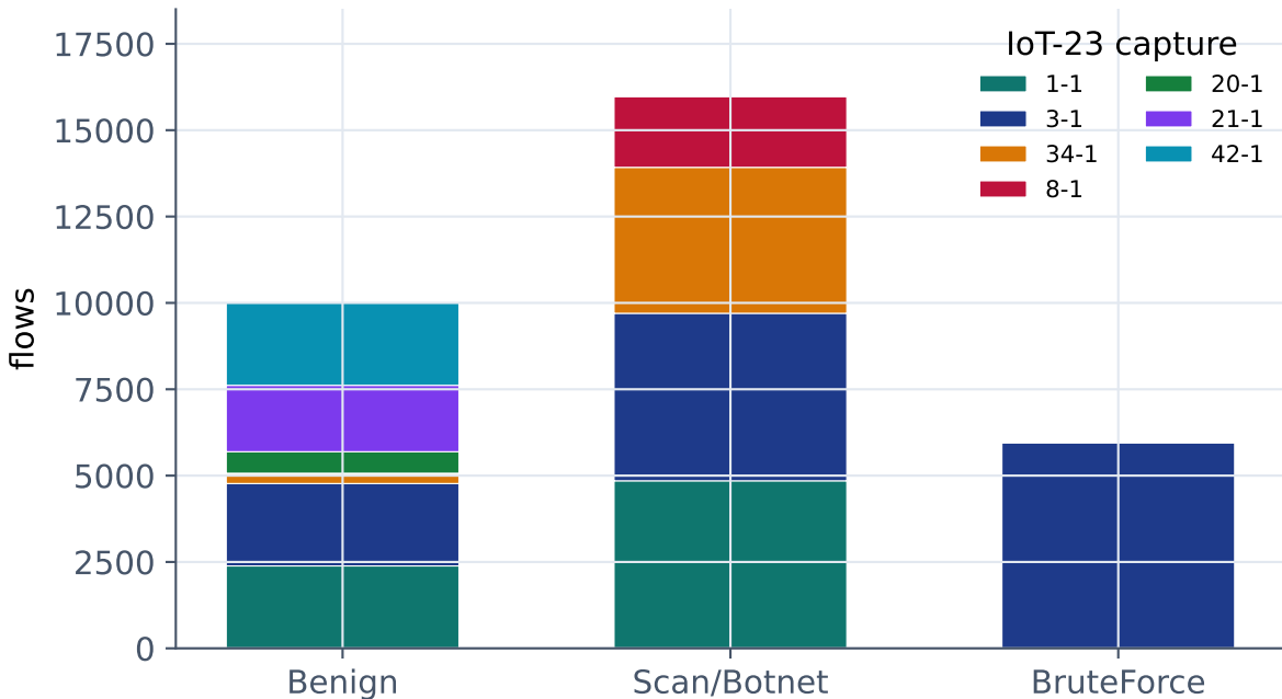
Training-set provenance — each class water-filled across captures
