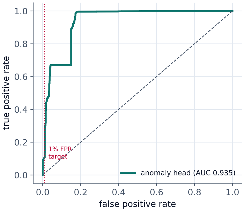
Anomaly head ROC (benign-trained, one-class)
