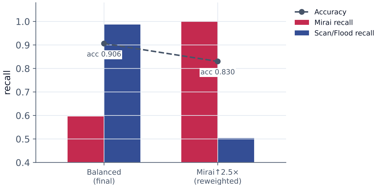
The see-saw: reweighting trades one class for another
