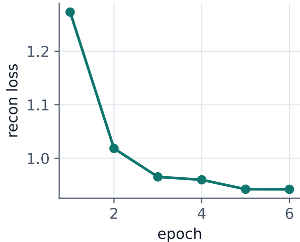
Stage A — SSL pre-train
