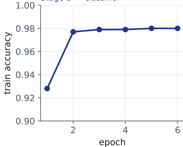
Stage B — classifier
