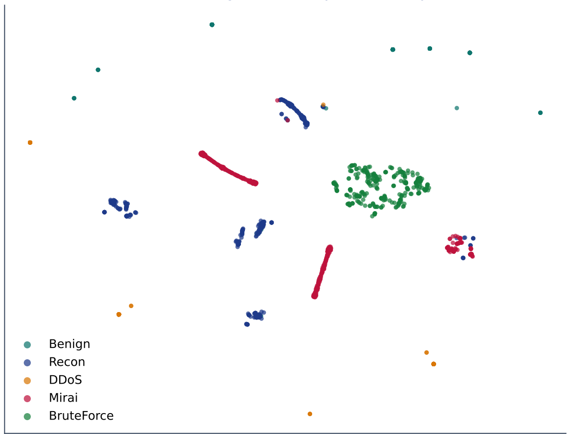
t-SNE of learned flow embeddings, coloured by attack family
