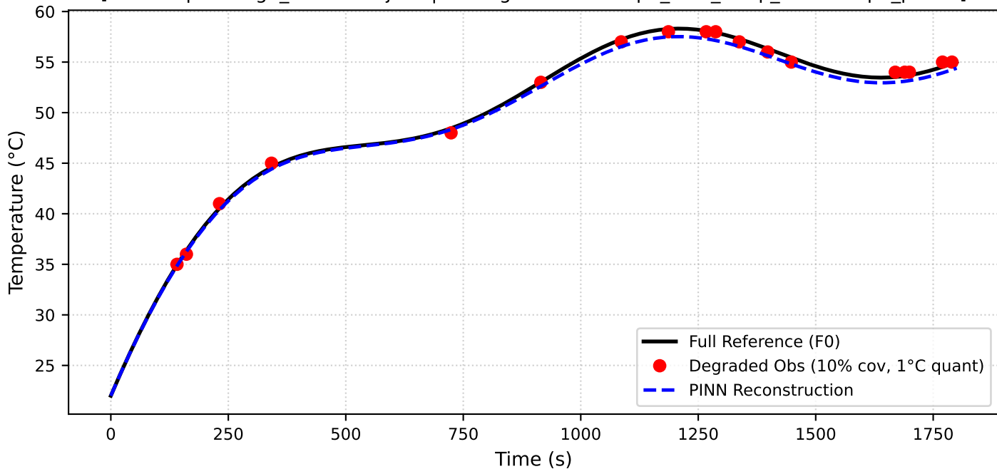
Fig 2. Representative Temperature Trajectory Reconstruction [Source: phase2g1_reference.json | Host: g04n06 GPU0 p0_core_temp_mean vs p0_power]
