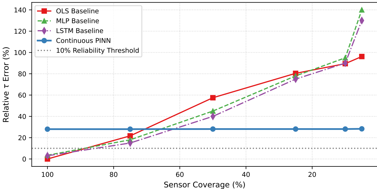
Fig 3. Thermal Parameter Recovery Error vs Sensor Coverage [Source: phase2g2_sparsity.json | Summit Hosts: g04n06, g14n16 GPU0]
