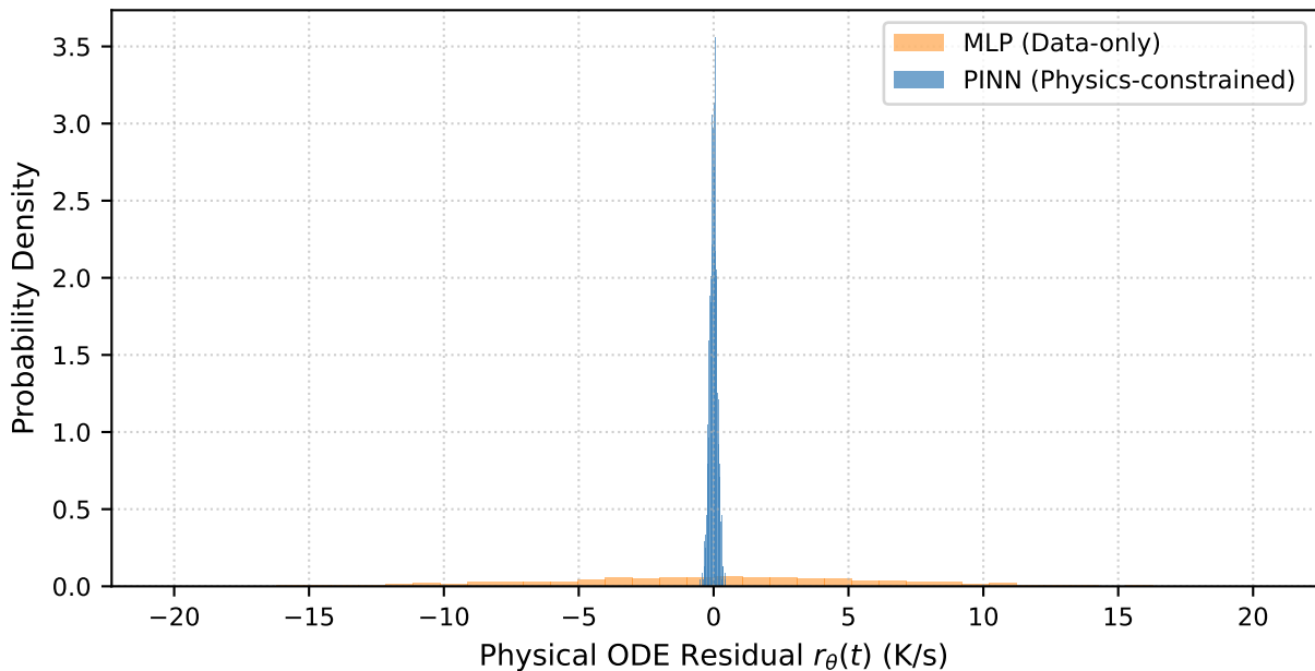
Fig 5. Physical ODE Residual Distribution Comparison [Source: ablation_data_vs_physics.json | Host: g04n06 GPU0]
