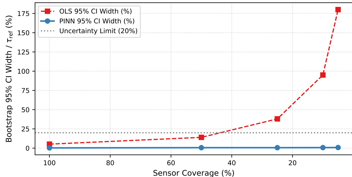
Fig 6. Parameter Uncertainty vs Telemetry Degradation [Source: phase2g5_combined.json | 2-Seed Bootstrap over Summit Hosts]
