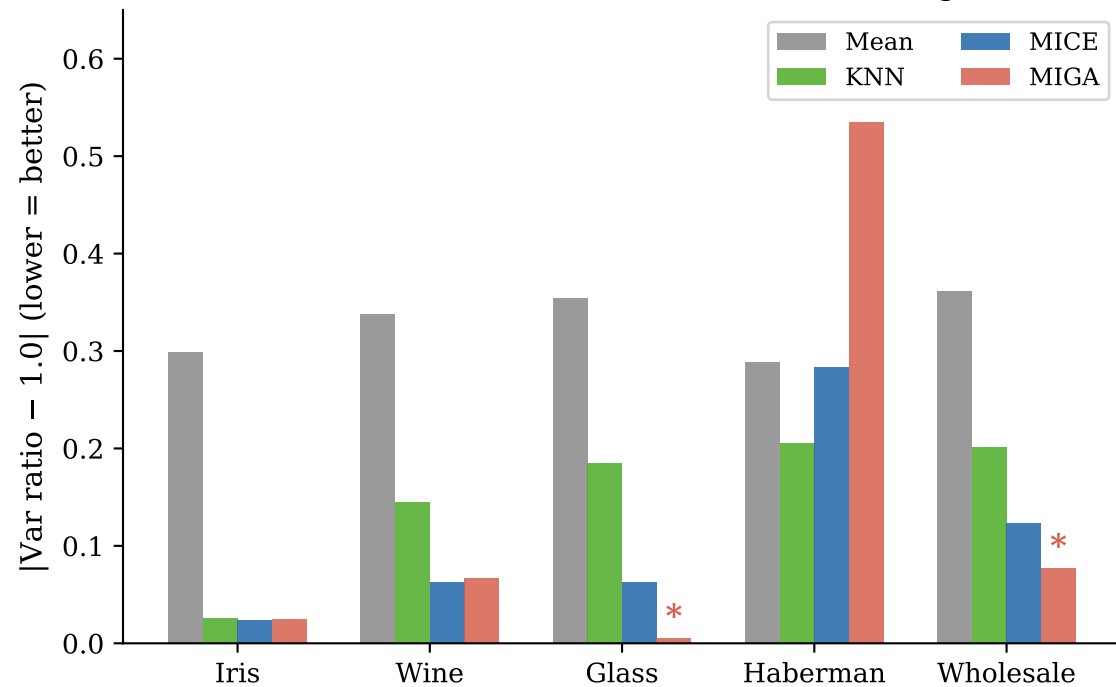
(a) Variance Preservation — 30% missing
