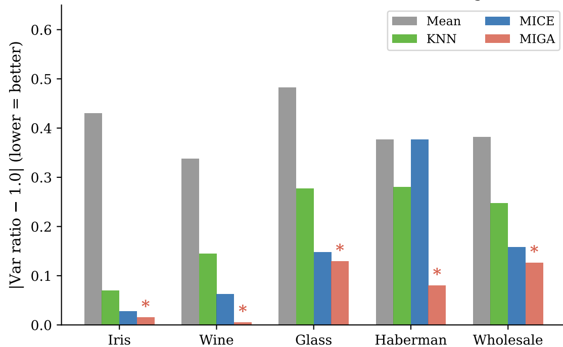
(b) Variance Preservation — 40% missing
