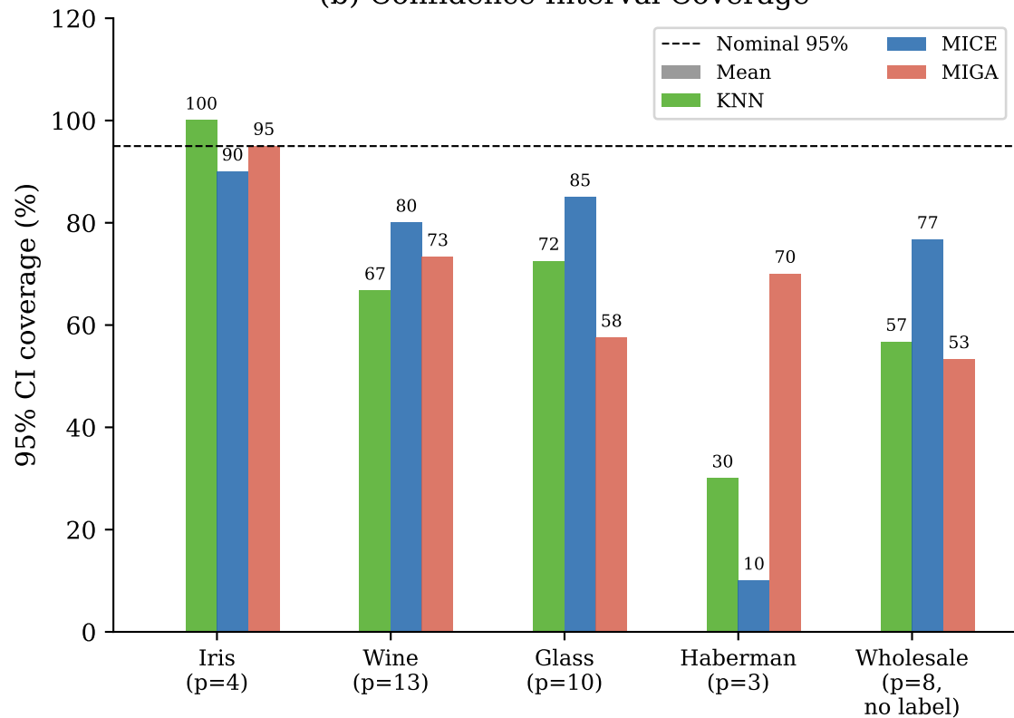
(b) Confidence Interval Coverage
