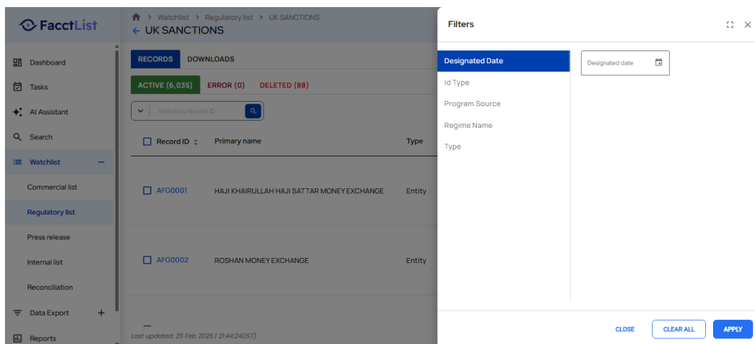
Screenshot: TestExecution_Step42_ACTION_Element.png
